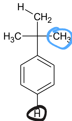
t -Butylbenzene
