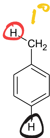
Toluene
