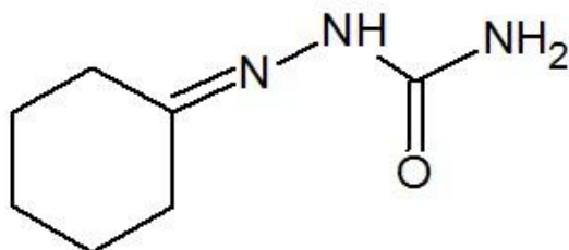
Cyclohexanone semicarbazone
