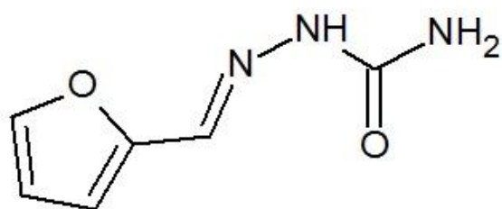
2-Furaldehyde semicarbazone
