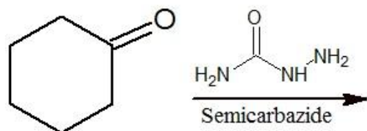
Cyclohexanone
