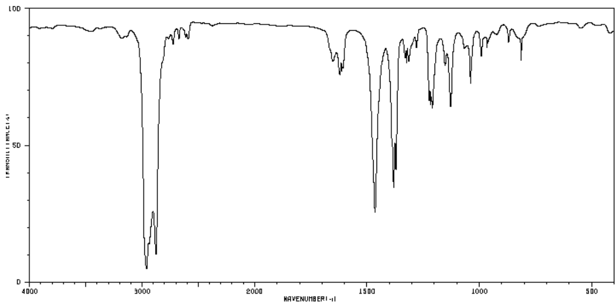
2,3-dimethylbutane
