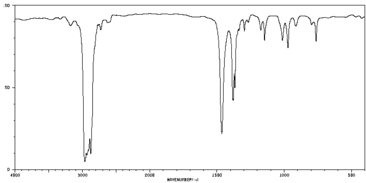
2-methylbutane
